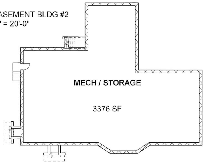
② FLOOR 1 BLDG #2 1" = 20'-0"
